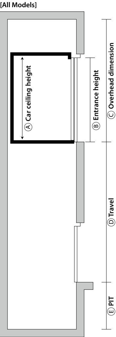
Elevation Plan
